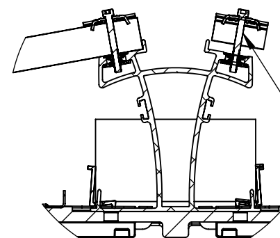
DETAIL G SCALE 2 : 13
