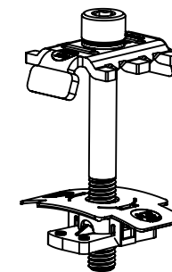
Bonding Mid Clamp
